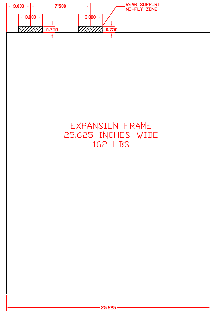
TOP VIEW
