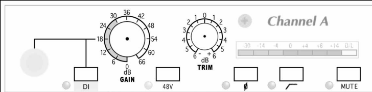
System 9098 Dual Mic Amplifier by Rupert Neve the designer
